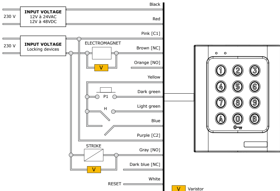
V Varistor
